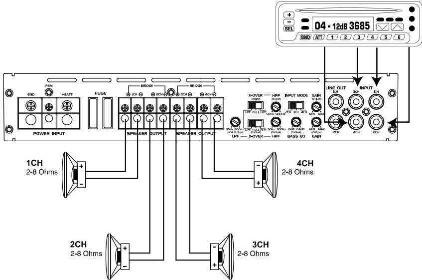
FIG. 7 4CHANNEL STEREO CONFIGURATION BAMF 1200/4, BAMF 1600/4
